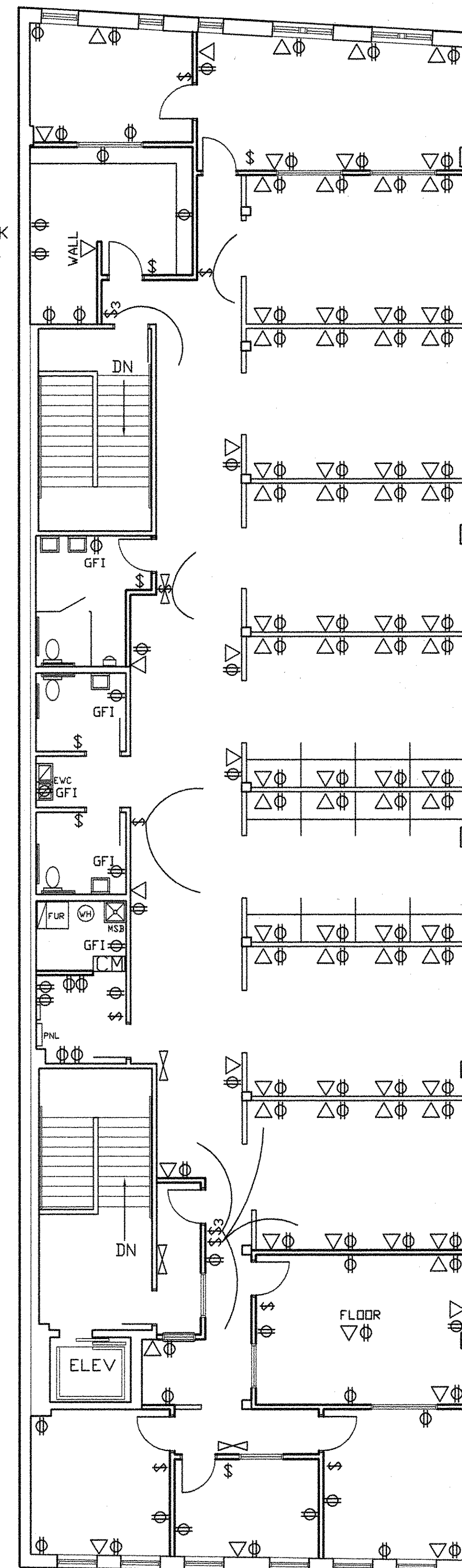
POWER PLAN
