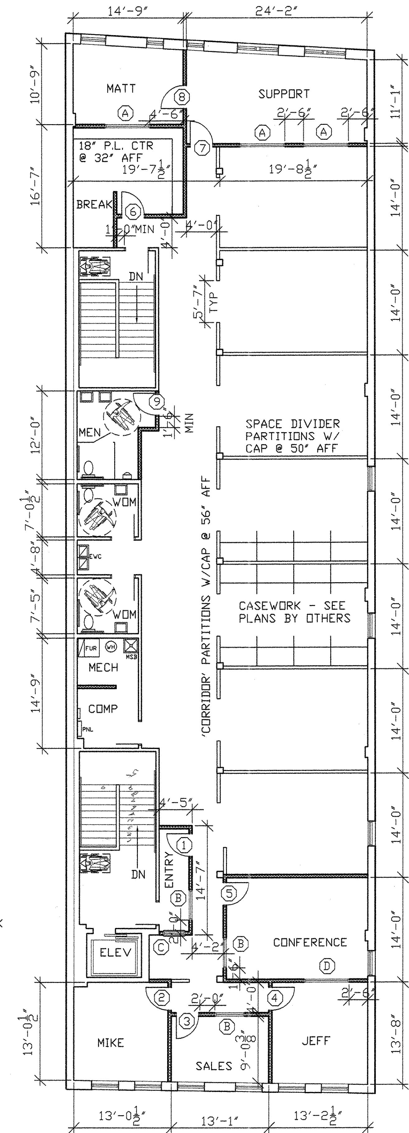
FLOOR PLAN
